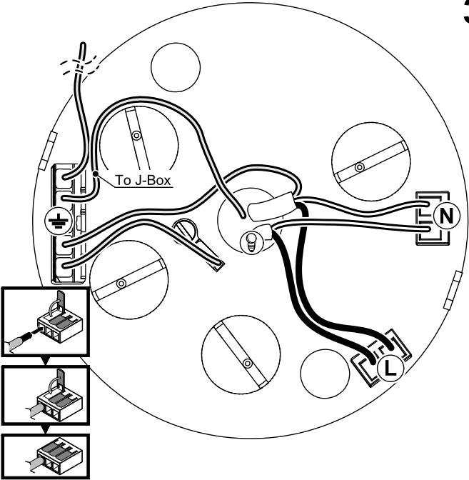
Detail 6
